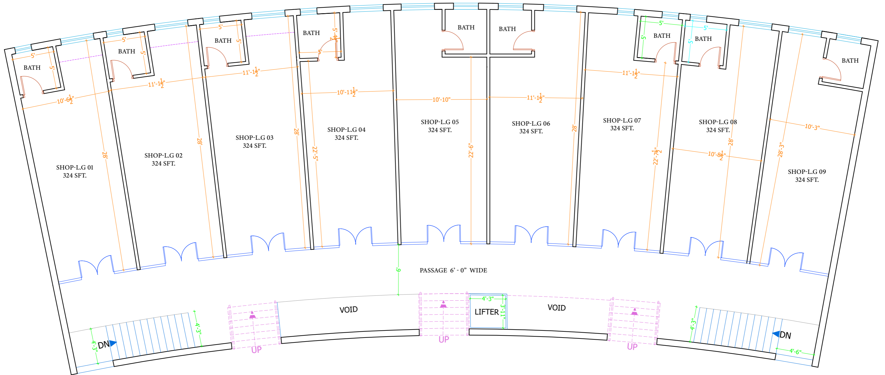
LOWER GROUND FLOOR PLAN
